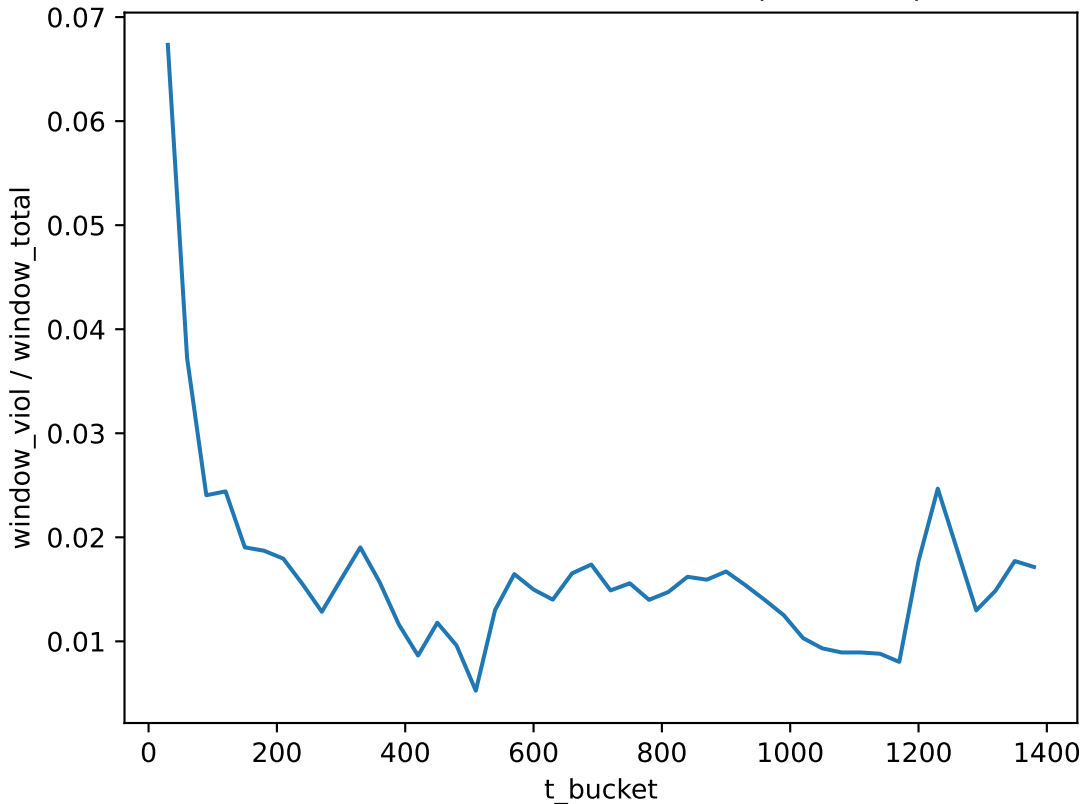
Cluster SLO violation fraction (balanced)
